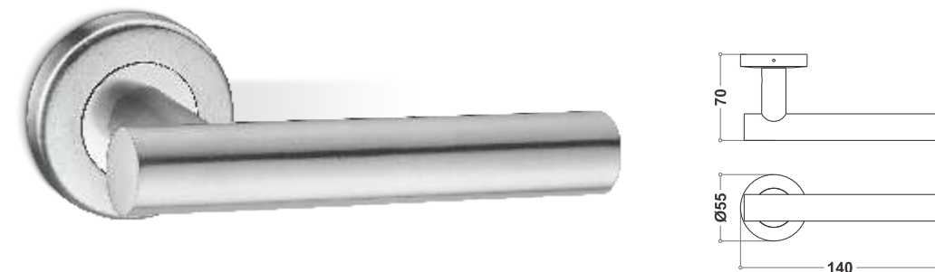
AMH-30 Mortise handle 22mm round pipe Finish : Satin / Glossy Material : Stainless steel 304 grade (Also available in plate type mortise)
