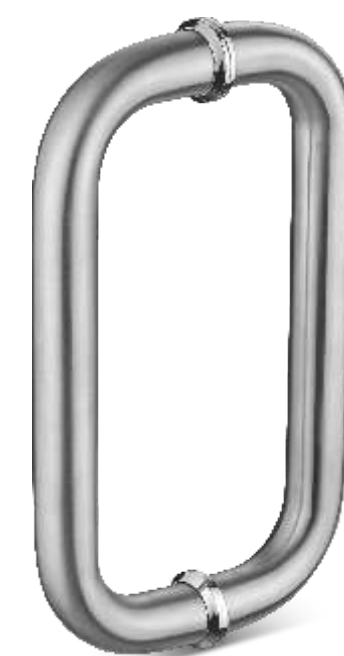
APH-06 D-type glass door handle Ø22mm / Ø25mm / Ø32mm pipe Finish : Satin / Combi Material : Stainless steel 304 grade
